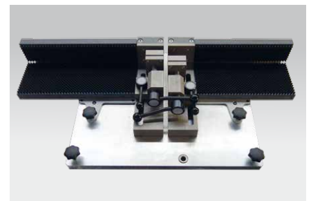
Quick-change clamping device with a manual vice for bar materials.
