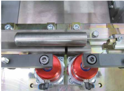
Prism tension via two pneumatic swing clamps (optional) and a digital workpiece stop.
