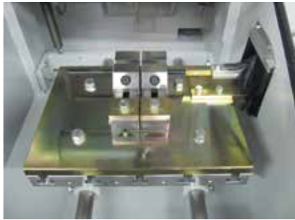
Parallel vices for material sizes between 2 – 20 mm with a digital workpiece stop.
