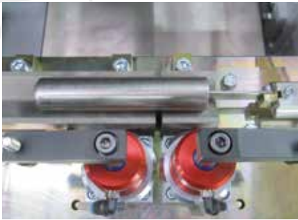
Prism tension via two pneumatic swing clamps and a digital workpiece stop.
